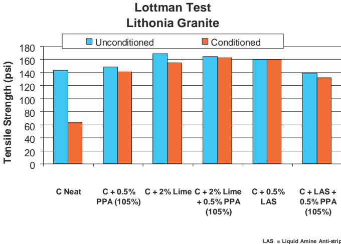
figure 5. Lottman Test Results of Binder with Lime and a Liquid Anti-strip Agent
