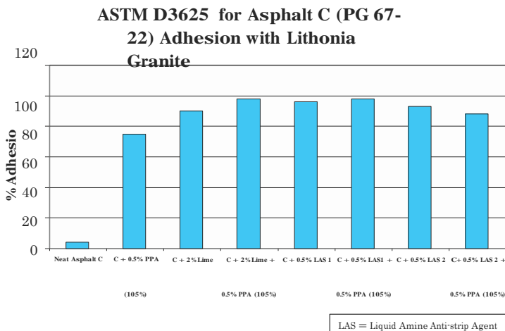
figure 3. Adhesion of Asphalt Binder to Lithonia Granite
